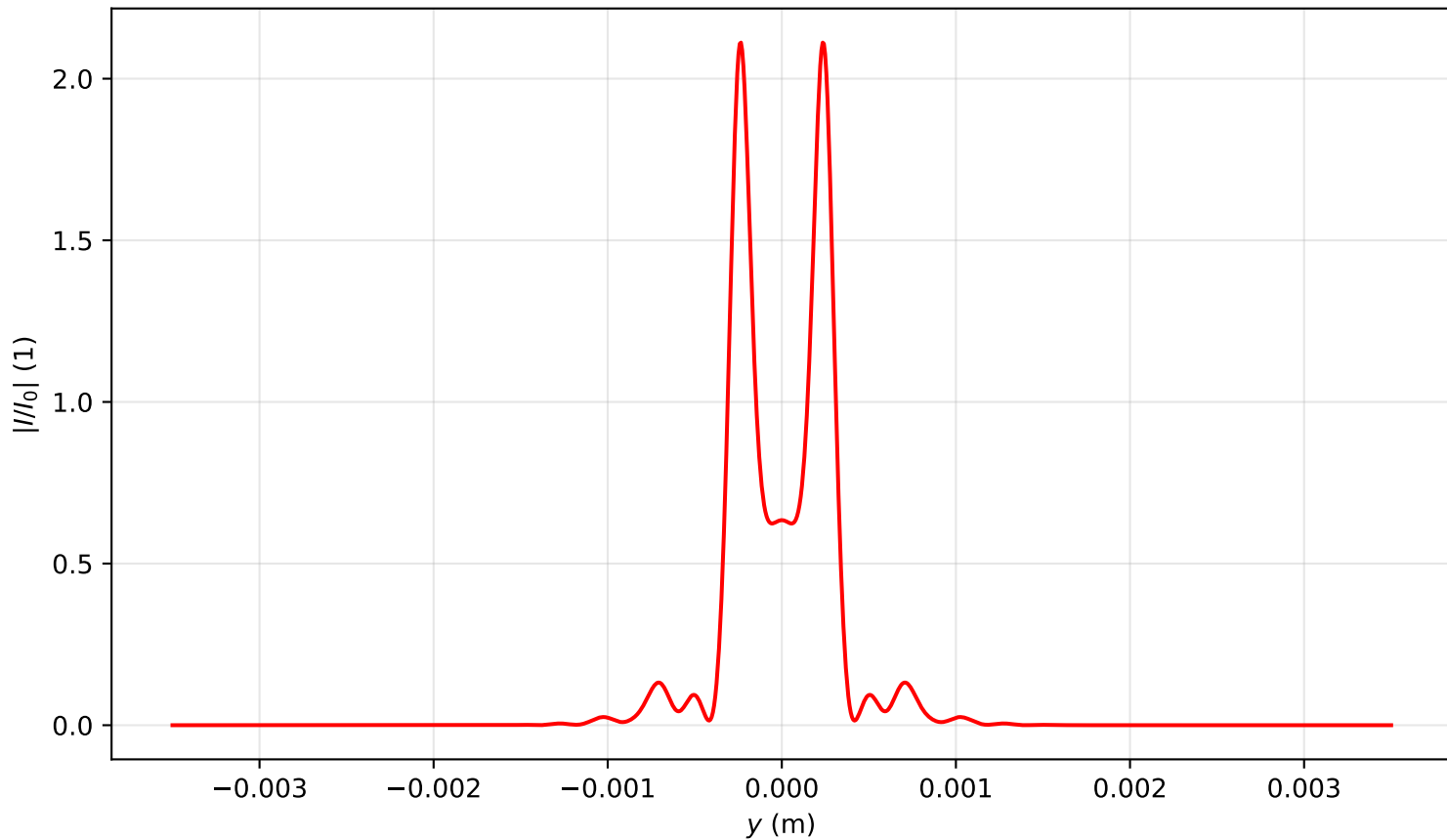
Intensity profile I(x = 0, y, z = 0.716)/I_0 , P_{in}=6.5P_{cr} , artificial time
